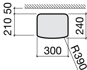
Diverta NR REF. A327114000
