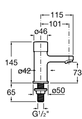
NR REF. A5A4224C00
