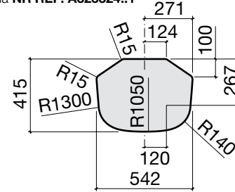
Dama NR REF. A325324..1
