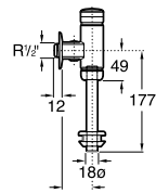
NR REF. A506902010
