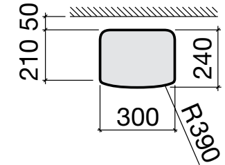
Diverta NR REF. A327114..0
