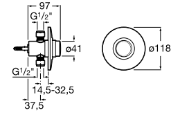
NR REF. A5A9024C00
