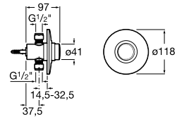
NR REF. A5A2624C00
