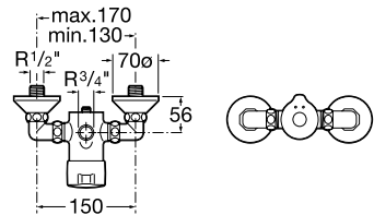
NR REF. A5A2117C00
